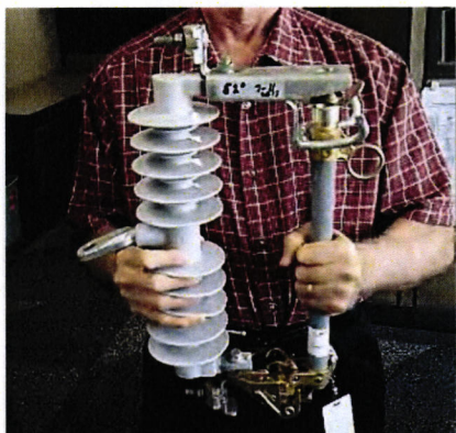
Fuse Link Assembly Cutout
