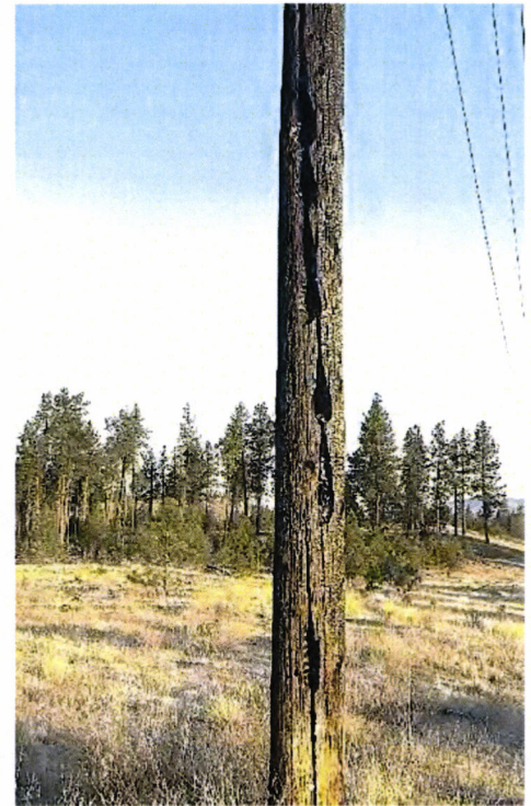
Pole fires generally occur on wood poles with wood crossarms. Since the early 2000's, Avista has adopted fiberglass crossarms as the standard unit. Replacing wood crossarms in elevated fire risk areas is a component of Wildfire Resiliency.
